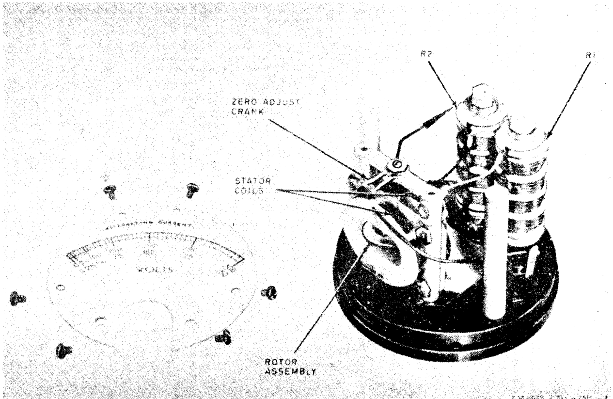
Figure 4. Voltmeter M2, AN/UPM-100, interior view.
